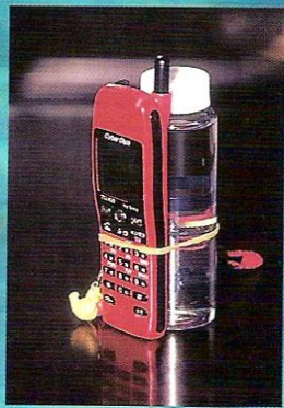
Water having received electromagnetic waves from a cellular phone
