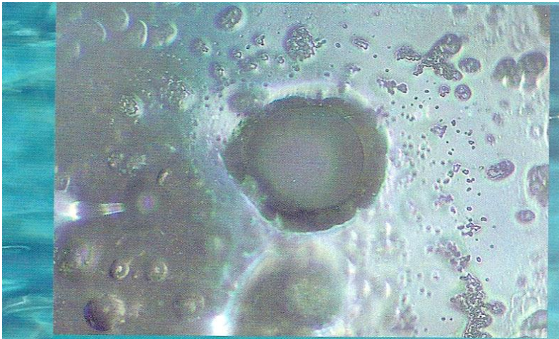
Water having received electromagnetic waves from a cellular phone
